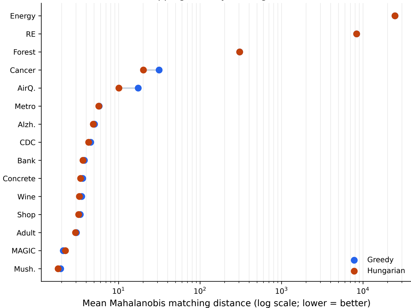
Mahalanobis mapping: Greedy → Hungarian (dataset means)
